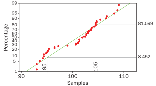
Figure 8. Comparing response from process capability reporting methods
